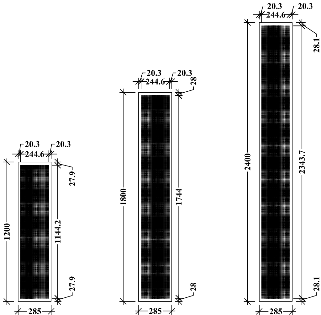
Quattro 75 with the actual size of 285 x 1200 mm, 285 x 1800 m and 285 x 2400 mm
