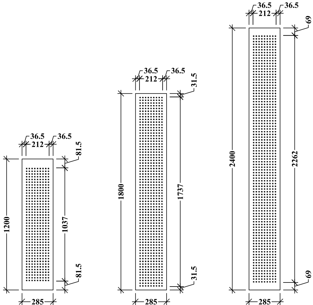
Quattro 55 with the actual size of 285 x 1200 mm, 285 x 1800 m and 285 x 2400 mm
