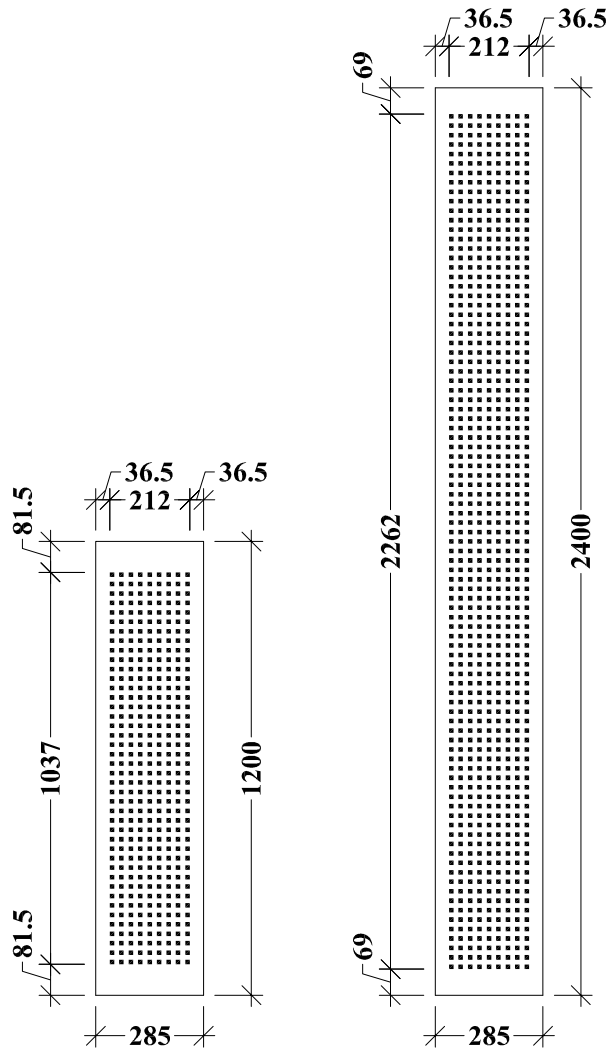
Xtensiv with the actual size of 285 x 1200 mm and 285 x 2400 mm
