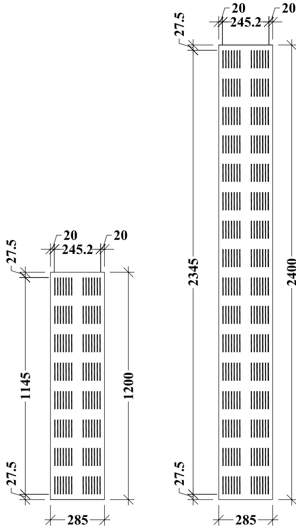
Xtensiv with the actual size of 285 x 1200 mm and 285 x 2400 mm
