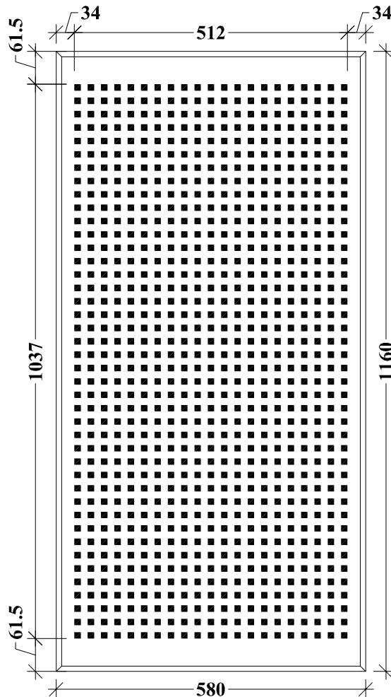
Trap modular size 580 x 1160 mm
