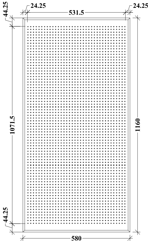
Trap modular size 580 x 1160 mm
