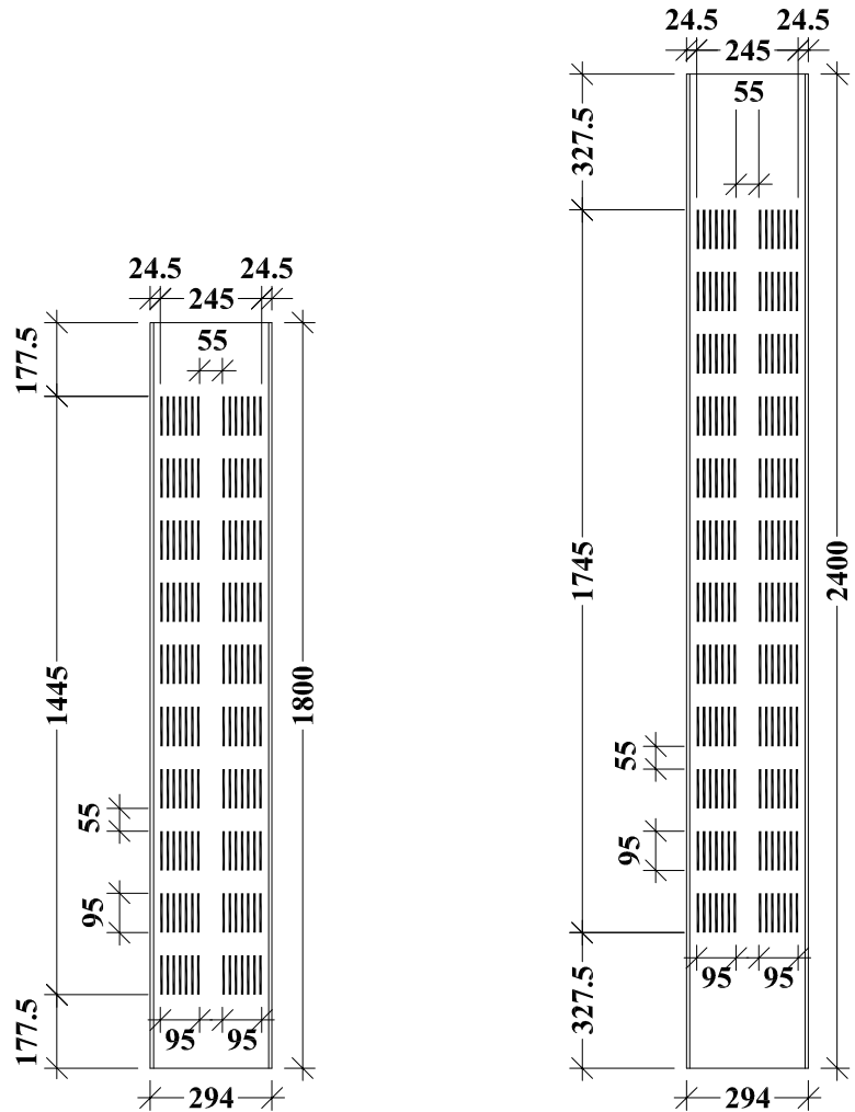
Plank with the actual size of 294 x 1800 mm and 294 x 2400 mm
