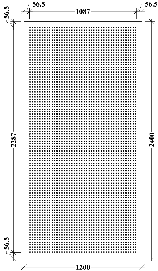
BIG Quattro 44 with the measurement of 1200 x 2400 mm
