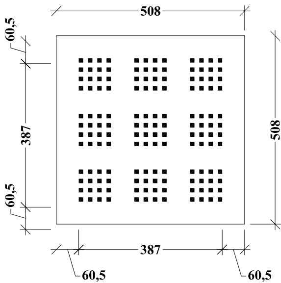
Access Panel Quattro 47 with the measurement of 508 x 508 mm
